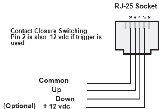
Figure 12: Pinout Diagram
